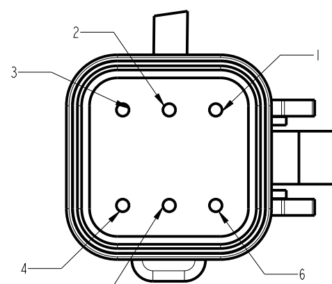
DETAIL G CONNECTOR A SCALE 2.000
