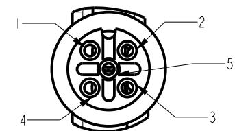
DETAIL A CONNECTOR A SCALE 2.000
