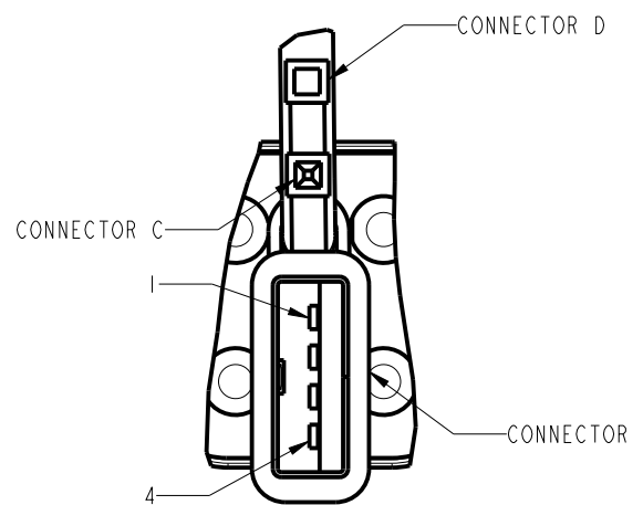
DETAIL I CONNECTOR B CONNECTOR C CONNECTOR D SCALE 2.000
