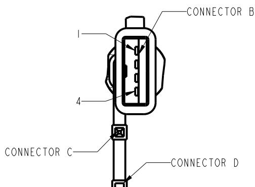
DETAIL B CONNECTOR B CONNECTOR C CONNECTOR D SCALE 1.500
